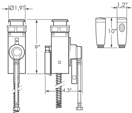
Retractable toilet jet for WC cleaning with 55" shower hose, hidden inside Armani Island collection built-in cabinet (Ref. A8164830..), sold as separate.
