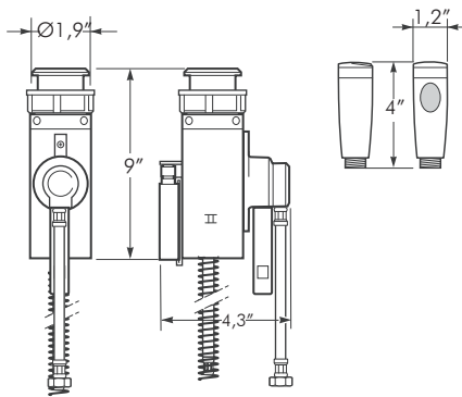
Retractable shower for intimate hygiene with 71" shower hose hidden inside Armani Island collection built-in cabinet (Ref. A8164830..), sold as separate.
